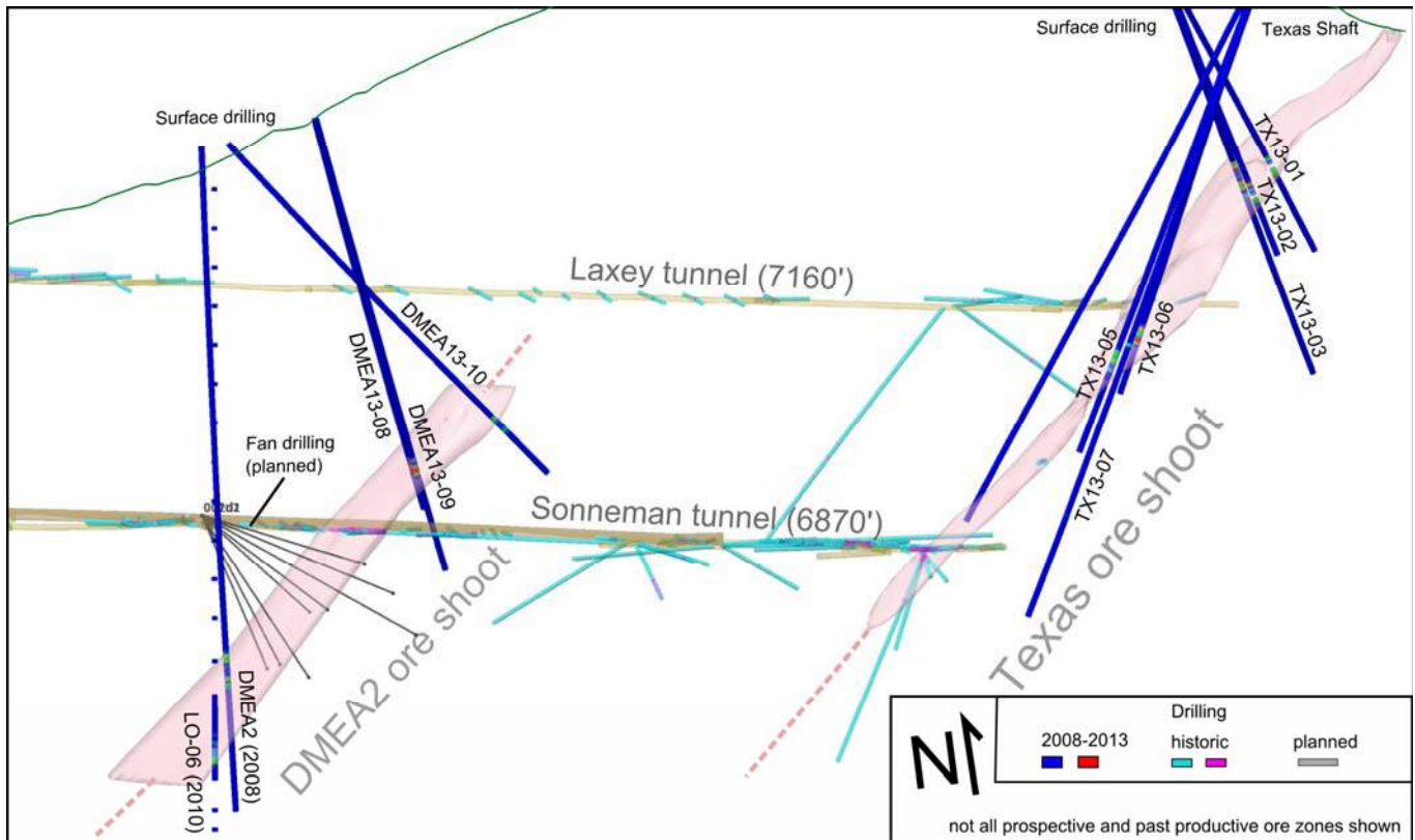
Long section looking north showing the Laxey and Sonneman tunnels and locations of some of the core drill holes.
